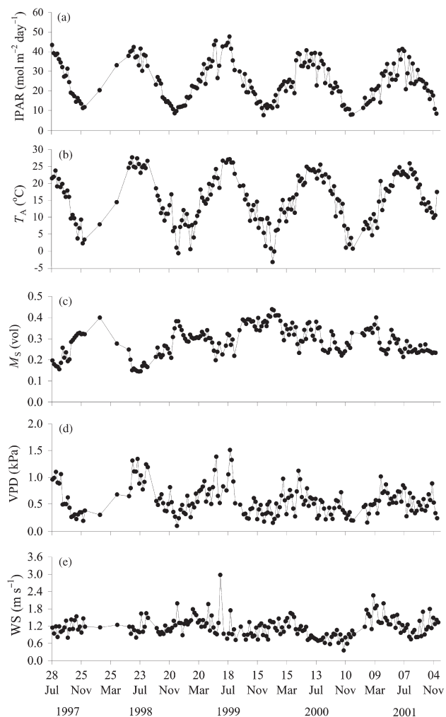
Figure 2. Change in climatic variables in the Duke Forest from August 1997 to December 2001. Abbreviations: IPAR = intercepted photosynthetically active radiation; M_S = soil water content; T_A = air temperature; VPD = vapor pressure deficit; and WS = wind speed.
