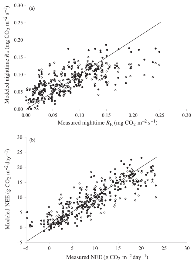
Figure 4. Comparison of model estimations and measurements of nighttime ecosystem respiration ( R_E ) (a) and net ecosystem exchange of carbon (NEE) (b). Symbols: \circ = values estimated by the multiple regression model; and \bullet = values estimated by the separate-slopes model.
