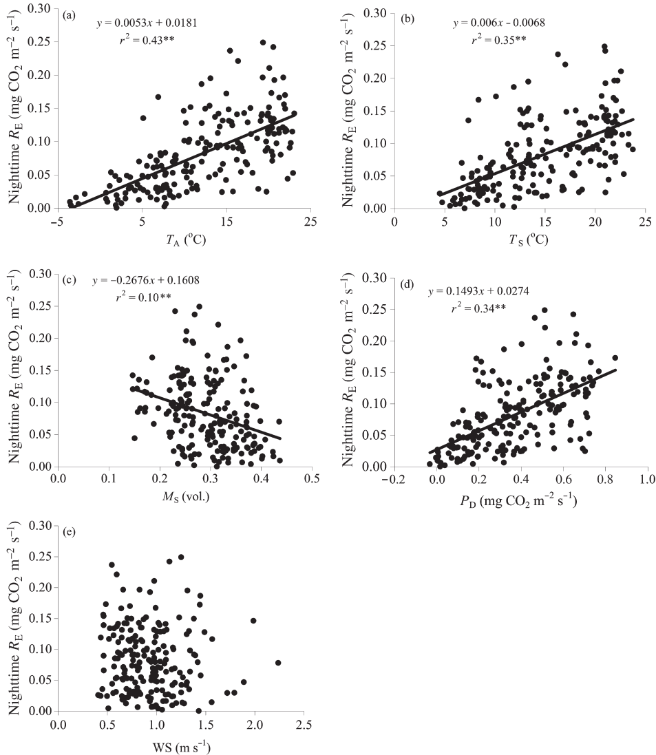
Figure 3. Relationships between nighttime R_E and the climatic variables ( M_S = soil water content; P_D = ecosystem CO 2 exchange; T_A = air temperature; T_S = soil temperature; and WS = wind speed). Double asterisks denote significance at the 0.01 level.
